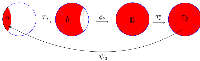
FIG. 2.2. Conformal equivalences from the disk
